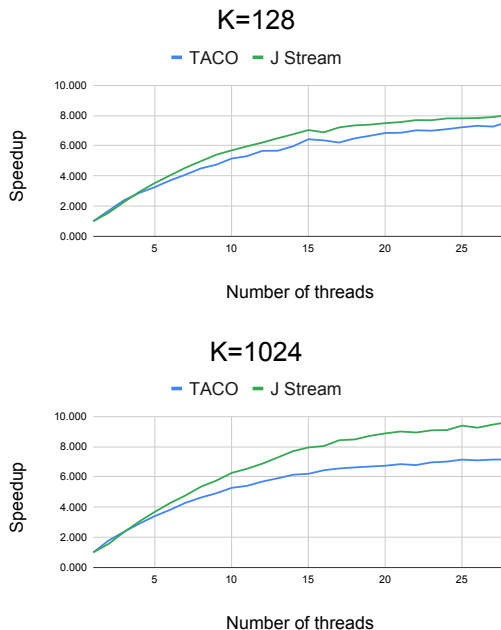
Fig. 8: SDDMM: speedup over single thread execution for TACO and J-Stream
