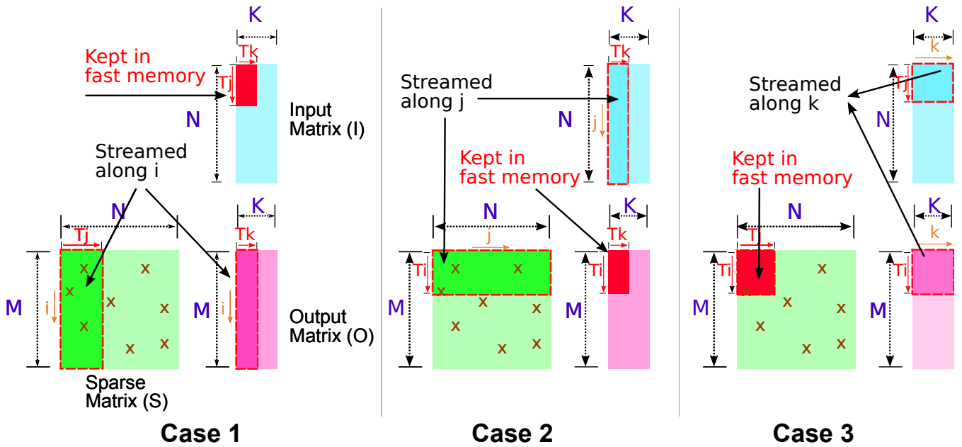
Fig. 2: Streaming SpMM.
