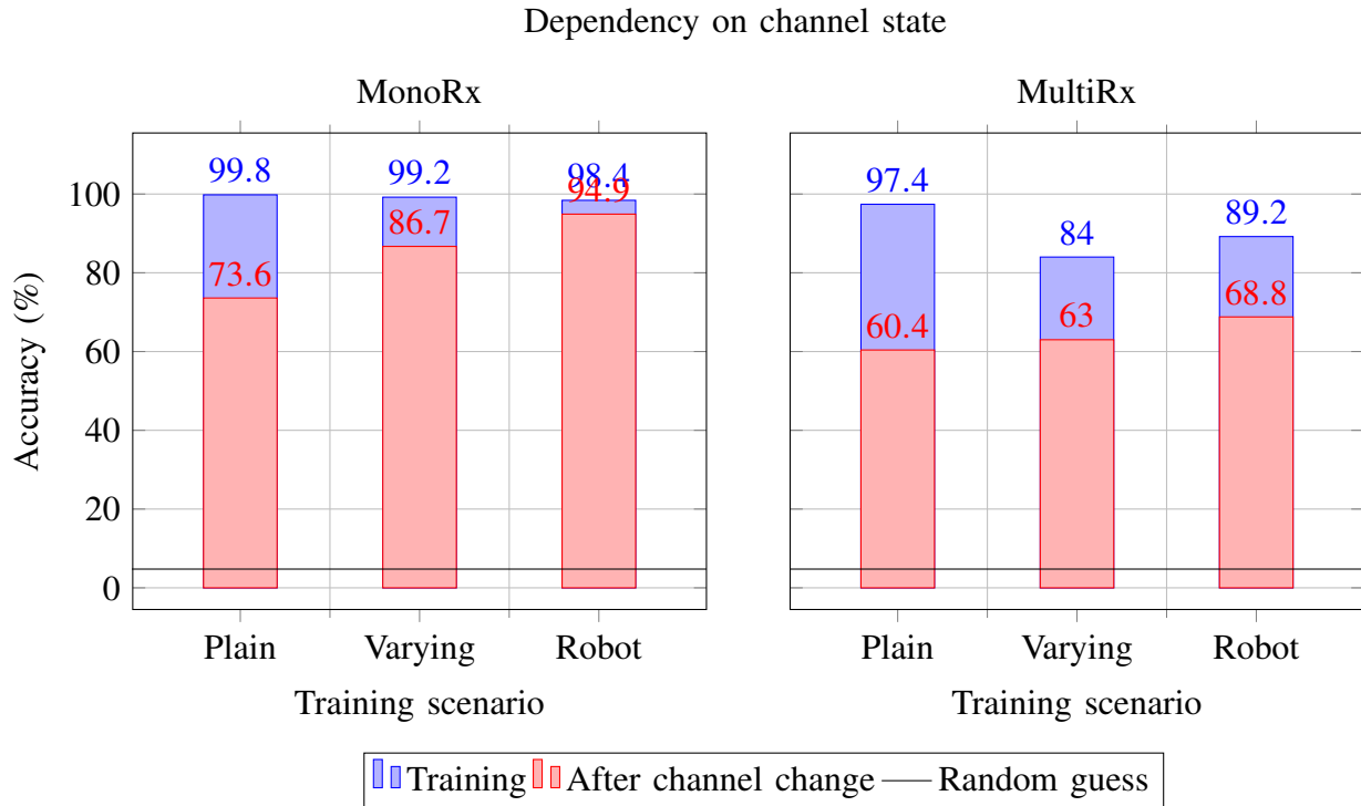
Fig. 11. Accuracy of networks trained on one scenario with static payloads and tested, either on data from the training dataset or on a dataset with the same scenario but with a modified environment.
