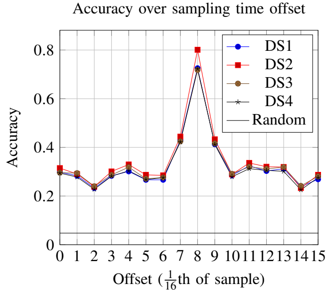
Fig. 13. Accuracy of a network trained on dataset 2 with an offset of eight and tested over the four datasets and 16 possible offsets
