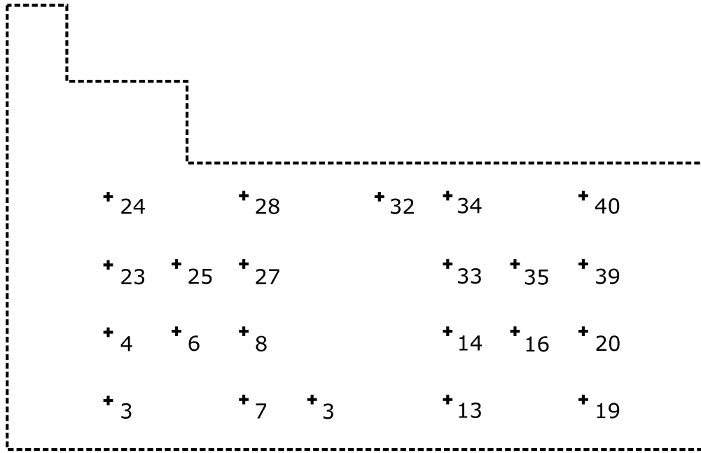
Fig. 3. FIT/CorteXlab experimentation room plan and node locations
