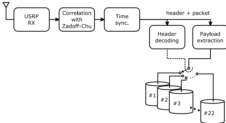
Fig. 6. Reception flowgraph.
