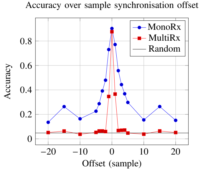
Fig. 12. Accuracy attained when the frame detector produces a timing offset
