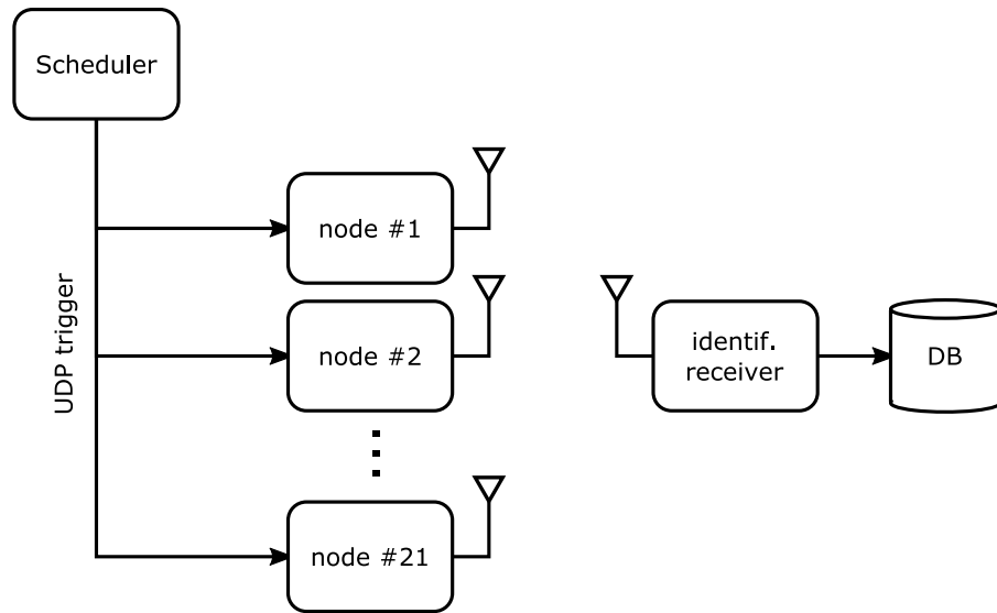
Fig. 4. Overall data collection topology (MonoRX)
