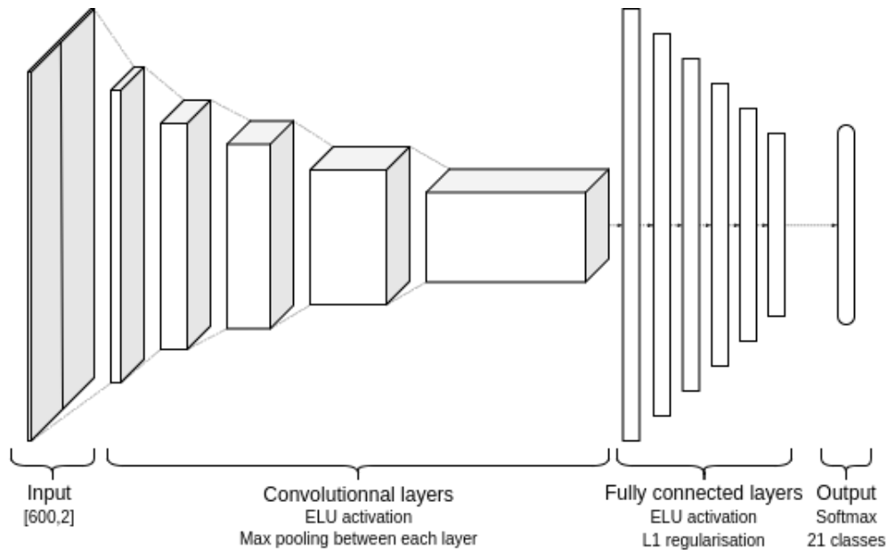
Fig. 8. Neural network architecture
