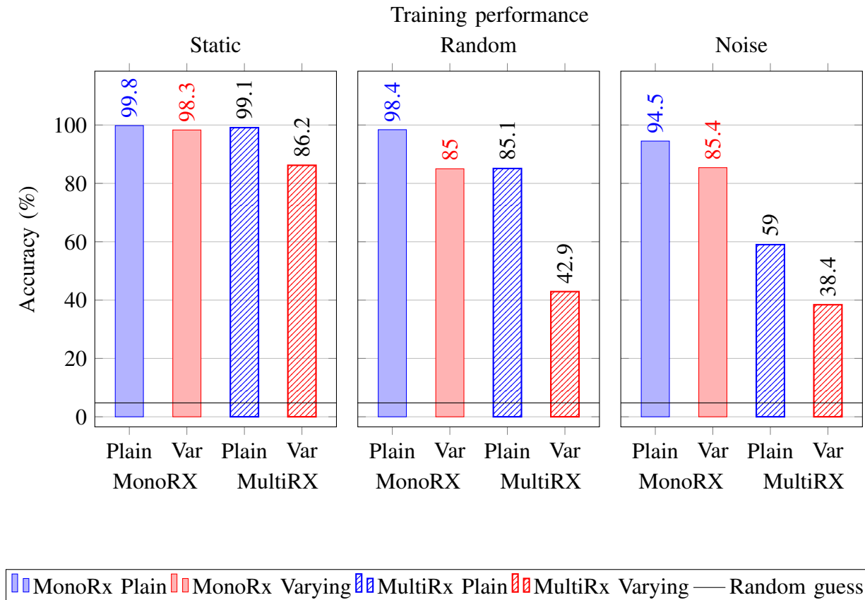
Fig. 9. Accuracy reached by networks trained on plain or varying amplitude scenarios and the 3 signal types. Accuracy is measured on the test set from the training dataset.
