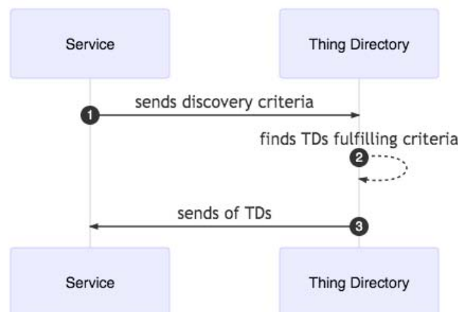
Figure 5.3.4-2: Thing discovery in WoT
