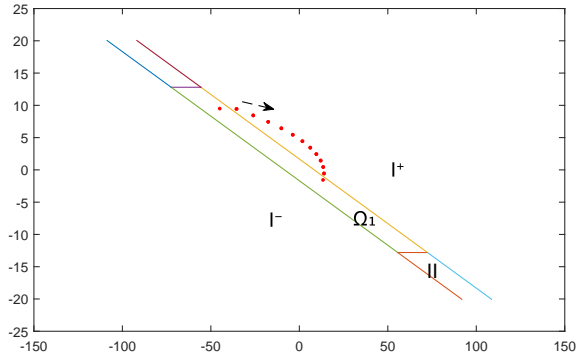
Fig. 5. The state trajectory of system (109) with x(0) = [-45, 9.5]^T .
