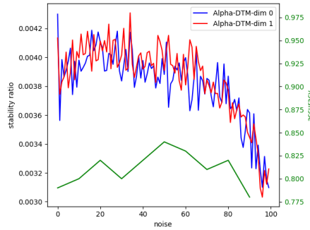
Figure 6: Empirical illustration of Multiparameter Persistence Image stability
