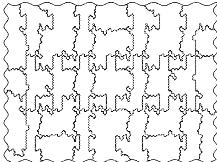
FIG. 7. 503,596 triangles agglomerated into 30 polygonal elements.
