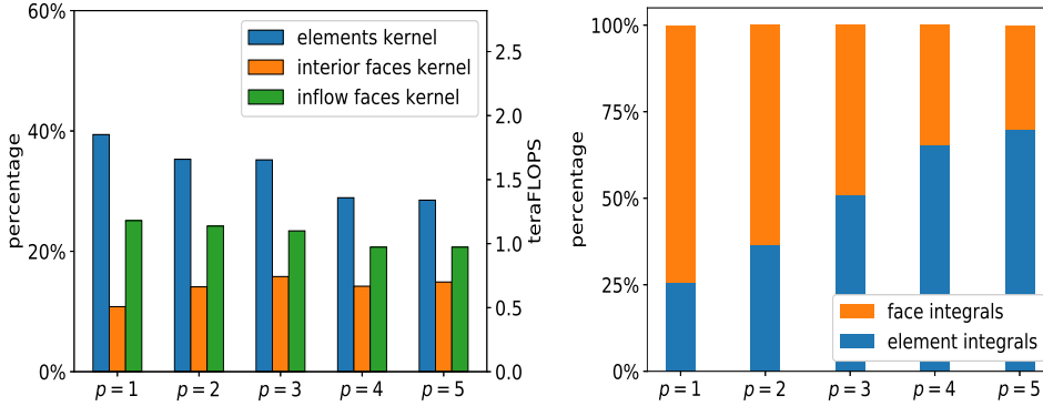
FIG. 6. Approach 2: (left) double precision performance percentage and FLOPS; (right) percentage of computation time for element vs. face kernels, for p = 1, \dots, 5 .
