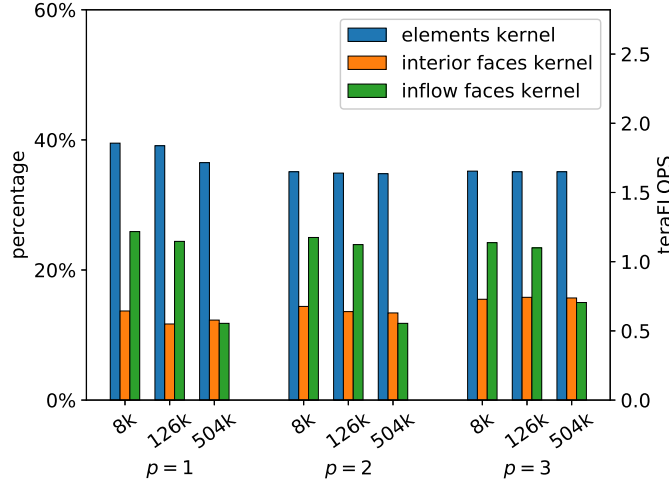
FIG. 8. Double precision performance of the three main kernels on the 3 meshes from Table 3, for p = 1, 2, 3 .
