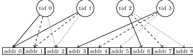
FIG. 5. Memory storage pattern of Approach 2 with scattered memory operations. Lines with same type are write operations that are performed simultaneously. Threads 0 and 1 are calculating integrals of the same polygonal element, hence they write in the same memory locations with atomic operations.
