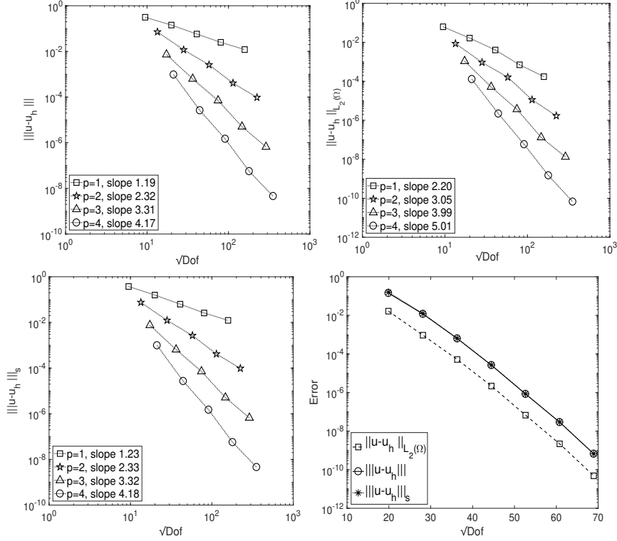
FIGURE 11. Example 2. Convergence history for p = 1, 2, 3, 4 , in \|\cdot\| (top-left), \|\cdot\|_{\Omega} (top-right) and \|\cdot\|_s (bottom-left) against \sqrt{\text{Dof}} for the meshes exemplified in Figure 10 with 30, 132, 555, 2151, 8337 elements, respectively. Bottom right: convergence history for p = 1, 2, \dots, 7 in the three norms against \sqrt{\text{Dof}} for the mesh with 132 elements shown in Figure 10 (right).
