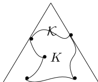
FIGURE 9. A simplex \mathcal{K} \in \mathcal{T}^\sharp covering an element K \in \mathcal{T} .
