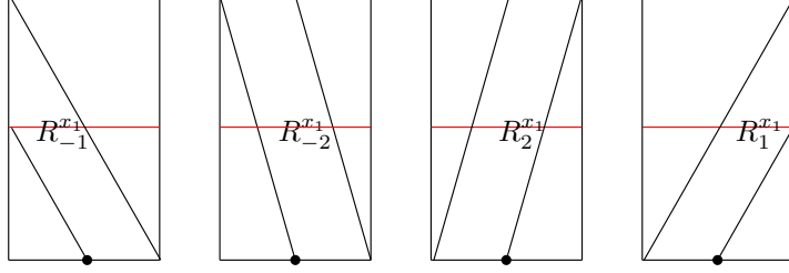
FIGURE 6. R = [0, 1] \times [0, 2] with subdivision R_i^{x_1} , i = -1, -2, 2, 1 .
