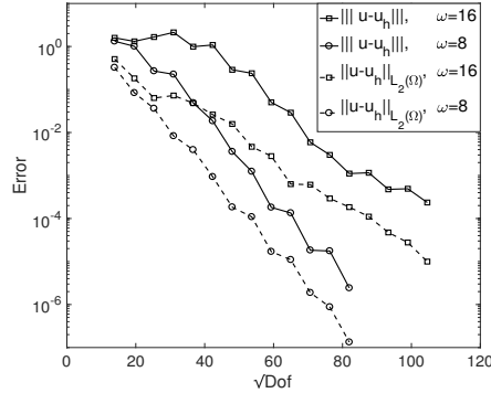
FIGURE 16. Example 4. Convergence history for p = 1, 2, \dots in the \|\cdot\| and \|\cdot\|_{\Omega} against \sqrt{\text{Dof}} for the curved triangular mesh with 64 elements shown in Figure 15, for A = 0.025 , \omega = 8, 16 .
