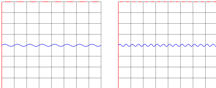
FIGURE 15. Example 4. The domain \Omega with the 64 element mesh fitted to the interface (blue) for A = 0.025 , and \omega = 8 (left) and \omega = 16 (right). The inflow parts of the boundary are drawn in red.
