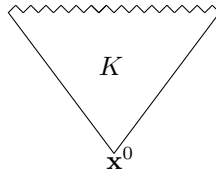
FIGURE 8. Example 4.26. K \in \mathcal{T} with ‘multiscale’ boundary behaviour.
