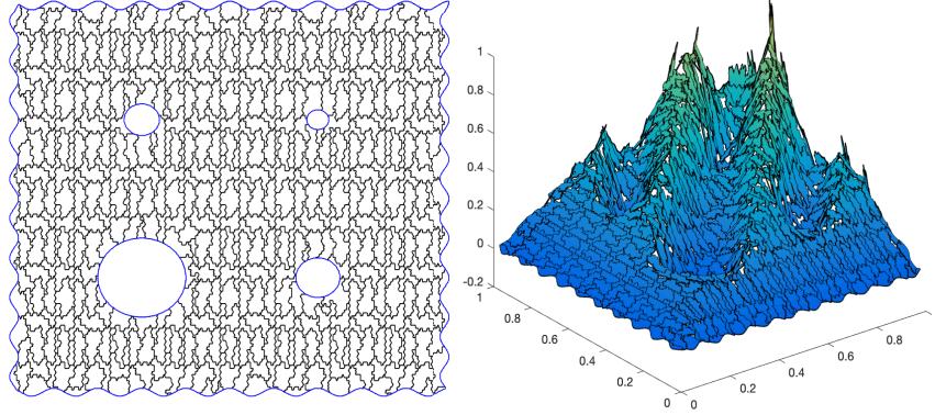
FIGURE 13. Example 3. Domain with holes and 531-element mesh (left). Corresponding solution obtained with p = 1 (right).
