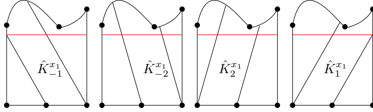
FIGURE 7. \hat{K}_i^{x_1} , i = -1, -2, 2, 1 for \hat{r} = 2 .
