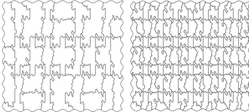
FIGURE 11. Example 2. The computational domain \Omega and two meshes with 30 and 132 elements, respectively.
