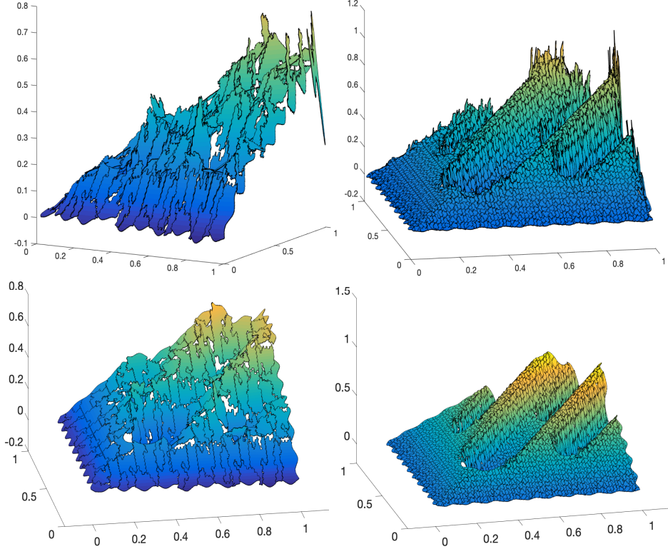
FIGURE 14. Example 3. Solutions computed for \epsilon = 10^{-4} (top) and \epsilon = 0 (bottom) using linear elements. The meshes are made of 129 (left) and 2048 (right) elements with complex shapes.
