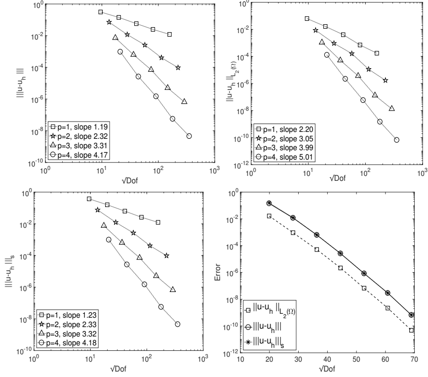
FIGURE 12. Example 2. Convergence history for p = 1, 2, 3, 4 , in |||\cdot||| (top-left), \|\cdot\|_{\Omega} (top-right) and |||\cdot|||_s (bottom-left) against \sqrt{\text{Dof}} for the meshes exemplified in Figure 11 with 30, 132, 555, 2151, 8337 elements, respectively. Bottom right: convergence history for p = 1, 2, \dots, 7 in the three norms against \sqrt{\text{Dof}} for the mesh with 132 elements shown in Figure 11 (right).
