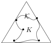
FIGURE 9. A simplex \mathcal{K} \in \mathcal{T}^\sharp covering an element K \in \mathcal{T} .
