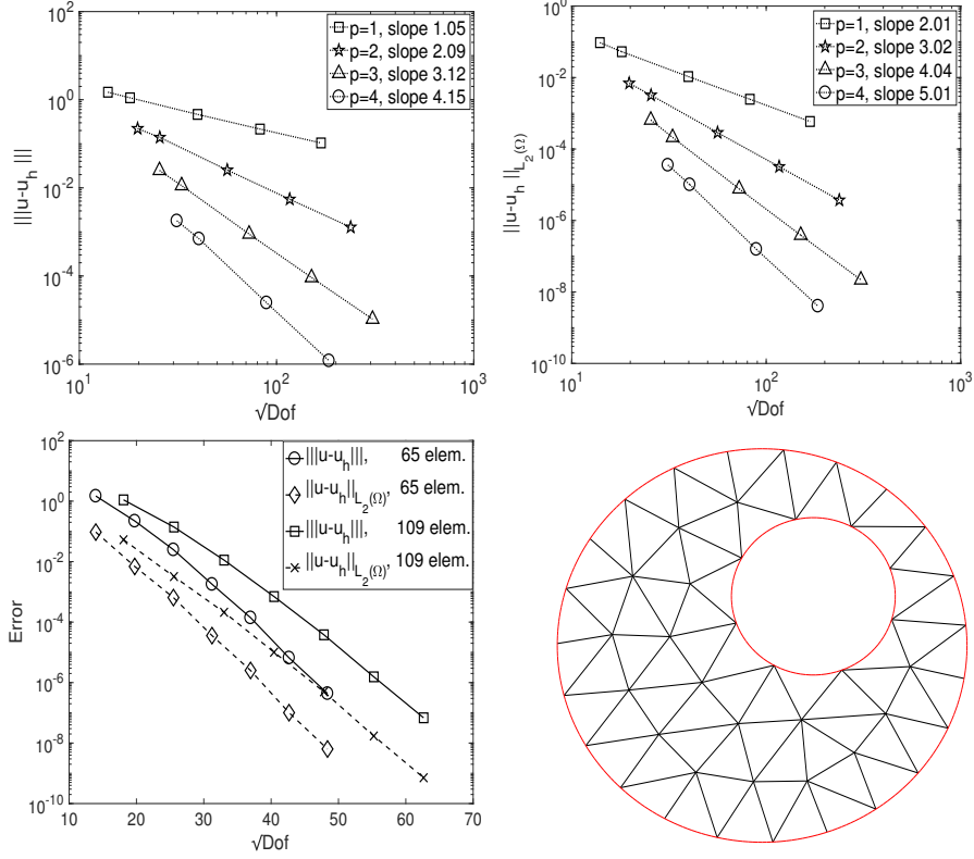
FIGURE 10. Example 1. Top: convergence history for p = 1, 2, 3, 4 in the \| | | \cdot \| | and \| \cdot \|_{\Omega} norms against \sqrt{\text{Dof}} for the curved triangular mesh exemplified in the bottom (right) plot with 65, 109, 527, 2266, and 9411 elements, respectively. Bottom (left): Convergence history for p = 1, 2, \dots, 7 in the \| | | \cdot \| | and \| \cdot \|_{\Omega} against \sqrt{\text{Dof}} for the meshes with 65 and 109 elements.
