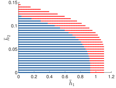
Fig. 9. Feasible values of \bar{h}_1 and \bar{h}_2 , when \bar{\eta}_1 = \bar{\eta}_2 = 0.075 , for the large-delay case (in blue) and the small-delay case (in red). For the small-delay case, the bounds \bar{h}_1 < 0.075 and \bar{h}_2 < 0.075 are applicable only if the condition (70) is satisfied.
