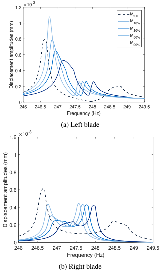
FIGURE 10: Displacements amplitudes at blades tip nodes for different masses of damper: Full damper, M = 90\%M_{full} , M = 50\%M_{full} , M = 30\%M_{full} , M = 10\%M_{full}
