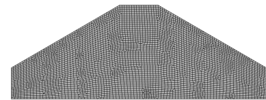
FIGURE 3: Mesh of the full damper
