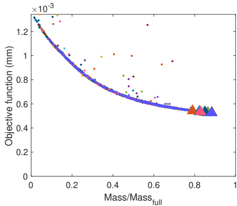
FIGURE 8: (a) Evolution of the objective function (i.e. max of displacements at blades tips) - (b) Objective function versus the normalized mass of the damper for all the different configurations tested during the algorithm
