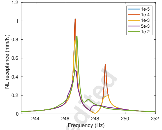
FIGURE 4: Nonlinear receptance at the point on the left blade for different excitation levels for a full damper
