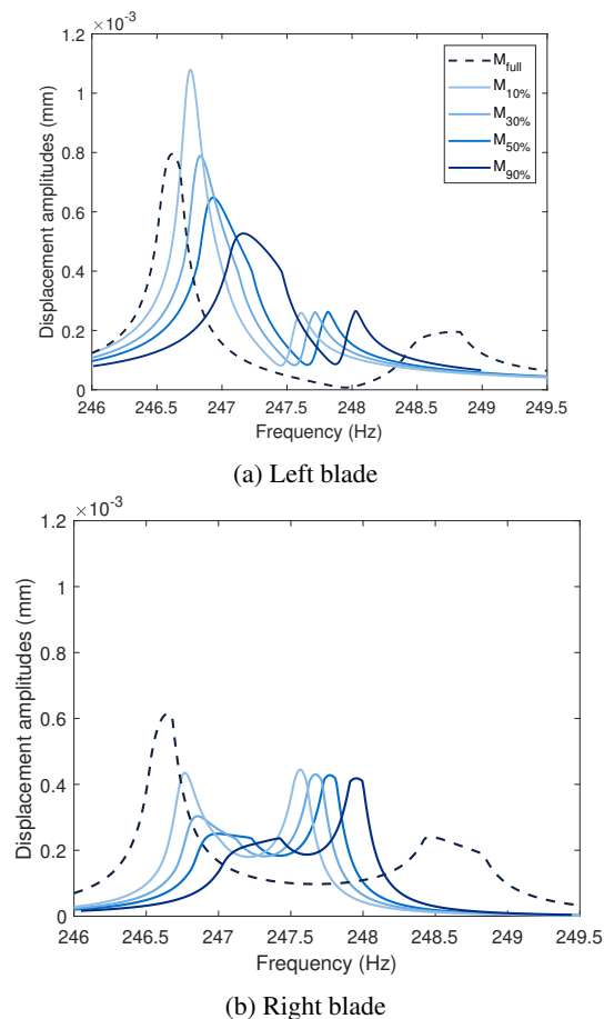
FIGURE 10: Displacements amplitudes at blades tip nodes for different masses of damper: Full damper, M = 90\%M_{full} , M = 50\%M_{full} , M = 30\%M_{full} , M = 10\%M_{full}
