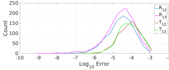
Figure 12. Errors of computed parameters w.r.t the GT are small showing that the solver is numerically stable of alternative formulation of Chicago
