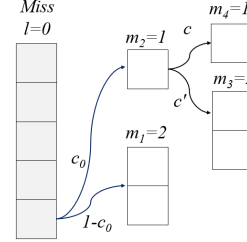
Fig. 2: Motivating example: a tree cache
