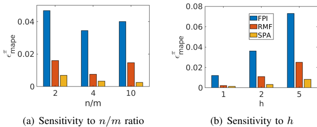
Fig. 6: Comparison between FPI, SPA and refined mean-field approximation (RMF) on models with random access probabilities.
