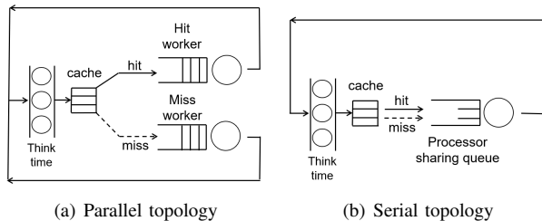
Fig. 8: Examples of models including a cache and queuing stations to model miss and fetch latencies. Routing and class-switching are state-dependent, since they depend on cache hits and cache misses.
