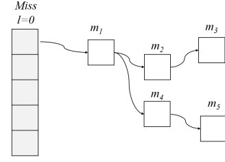
Fig. 5: A tree cache with h = 5 lists. List capacities vary between m_j = 1 and m_j = 50 .
