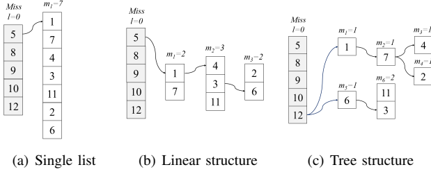
Fig. 1: Examples of list-based caches with different internal structure, total capacity m = 7 , and n = 12 items.
