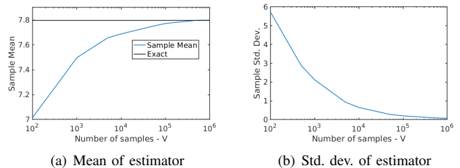
Fig. 10: Convergence of Monte Carlo estimator for E(\mathbf{m}, \mathbf{k})
