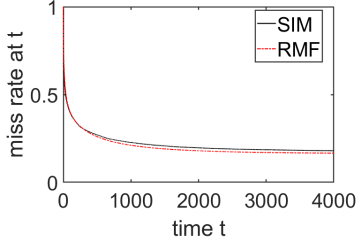
Fig. 3: RMF transient analysis for n = 50
