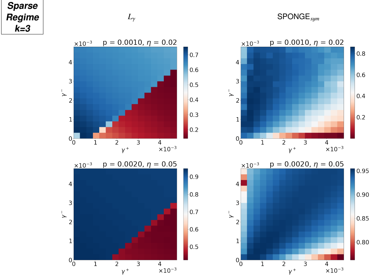
Figure 4: Heatmaps of the Adjusted Rand Index between the ground truth and the partition obtained using the L_\gamma and \text{SPONGE}_{sym} algorithm with fixed parameters ( \tau^+ , \tau^- ) and varying regularization parameters ( \gamma^+ , \gamma^- ), for a SSBM in two sparse regimes, with n = 5000 and k = 3 clusters.
