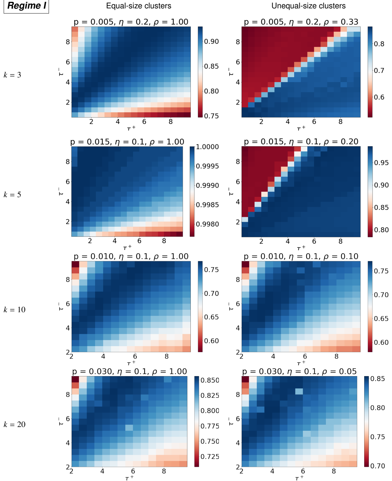
Figure 1: Heatmaps of the Adjusted Rand Index between the ground truth and the partition obtained using the SPONGE sym algorithm with varying regularization parameters ( \tau^+, \tau^- ), for a SSBM in Regime I, with n = 5000 and k = \{3, 5, 10, 20\} clusters of equal sizes (left column) and unequal sizes (right column).
