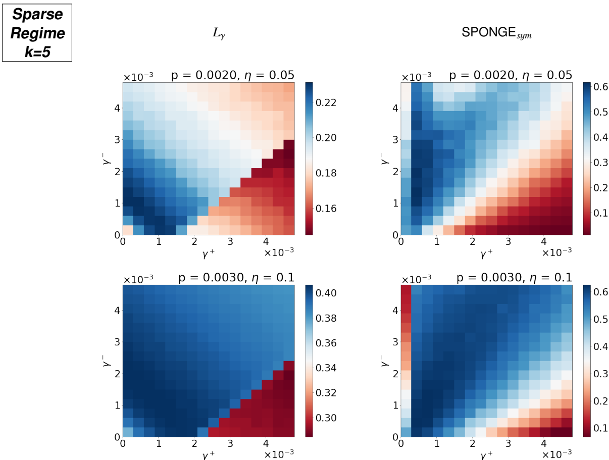
Figure 5: Heatmaps of the Adjusted Rand Index between the ground truth and the partition obtained using the L_\gamma and \text{SPONGE}_{sym} algorithm with fixed parameters ( \tau^+ , \tau^- ) and varying regularization parameters ( \gamma^+ , \gamma^- ), for a SSBM in two sparse regimes, with n = 5000 and k = 5 clusters.
