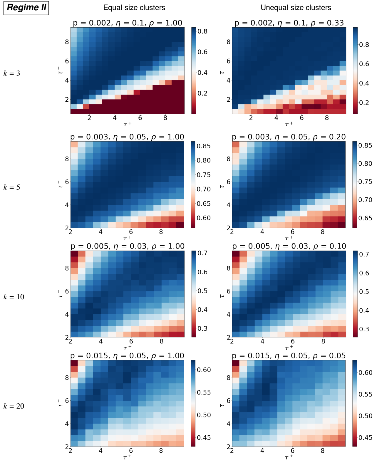
Figure 2: Heatmaps of the Adjusted Rand Index between the ground truth and the partition obtained using the \text{SPONGE}_{sym} algorithm with varying regularization parameters ( \tau^+, \tau^- ), for a SSBM in Regime II with n = 5000 and k = \{3, 5, 10, 20\} clusters of equal sizes (left column) and unequal sizes (right column).
