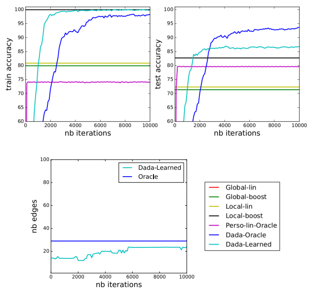
Figure 1: Results on the Moons dataset. Top : Training and test accuracy w.r.t. iterations (we display the performance of non-collaborative baselines at convergence with a straight line). Global-lin is off limits at \sim 50\% accuracy. Bottom : Average number of neighbors w.r.t. iterations for Dada-Learned.
