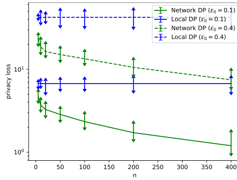
Figure 3: Comparing network and local DP on the task of computing discrete histograms. The results are obtained for T = 100n (i.e., the expected number of contributions per user is 100). The value of \epsilon_0 rules the amount of local noise added to each contribution (i.e., each single contribution taken in isolation satisfied \epsilon_0 -LDP). Curves report the average privacy loss across all pairs of users and all 10 random runs, while their error bars give the best and worst cases.
