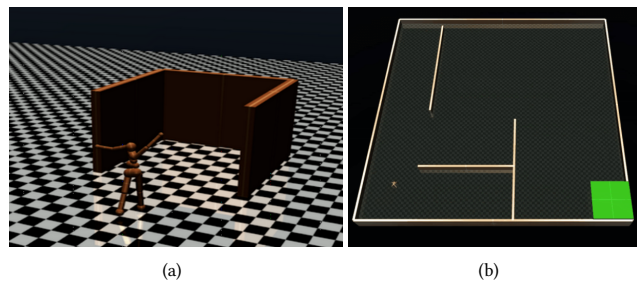
Figure 4: Domains for the deep exploration study. a: Deceptive Humanoid domain. b: Ant Maze domain. Here the goal is the green area and the trap is in the cul-de-sac to the right of the agent’s starting position.
