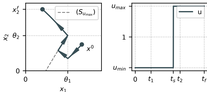
Fig. 2. Optimal trajectory with x_1^0 = 0.8 , x_2^0 = 0.3 and x_2^f = 0.7 . Times t_1 and t_2 are the transition times at which the state meets x_1(t_1) = x_1(t_2) = \theta_1 and x_2(t_2) = \theta_2 .
