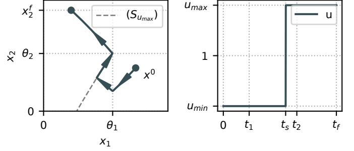
Fig. 2. Optimal trajectory with x_1^0 = 0.8 , x_2^0 = 0.3 and x_2^f = 0.7 . Times t_1 and t_2 are the transition times at which the state meets x_1(t_1) = \theta_1 and x_2(t_2) = (\theta_1, \theta_2) .
