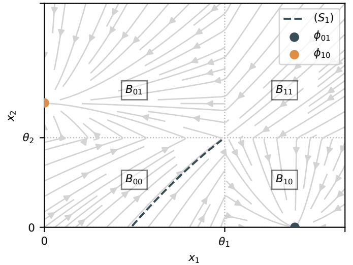
Fig. 1. Stream plot with free dynamics. System parameters are \gamma_1 = 1.2 , \gamma_2 = 1.8 , \theta_1 = 0.6 , \theta_2 = 0.4 , k_1 = k_2 = 1 .
