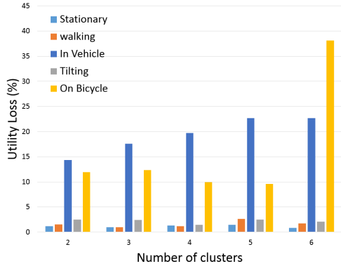
Fig. 3: Utility loss per activity wrt number of clusters
