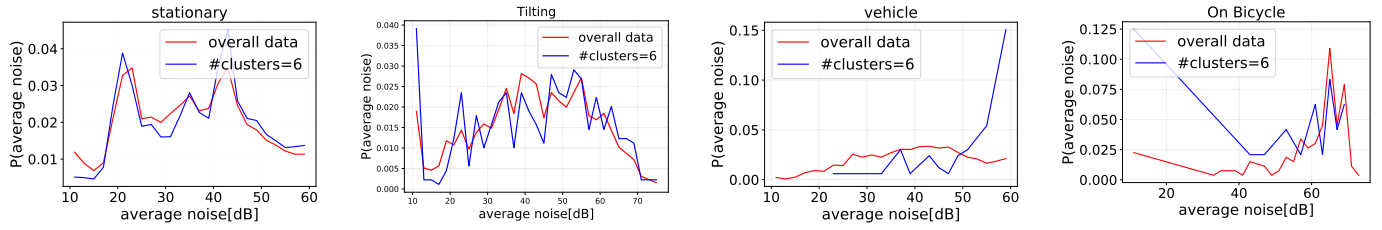
Fig. 4: Distribution of the collected values per activity after clustering
