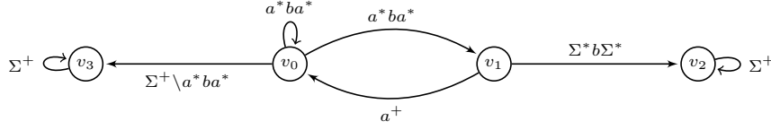
■ Figure 5 Parameterized arena for the synthesis of a coalition strategy.
