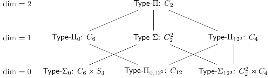
FIGURE 3. The taxonomy of reduced automorphism groups of elliptic products. Dimensions on the left are of the loci on each level in the 3-dimensional moduli space of PPASes. Lines connect sub-types and super-types; specialization moves down the page.
