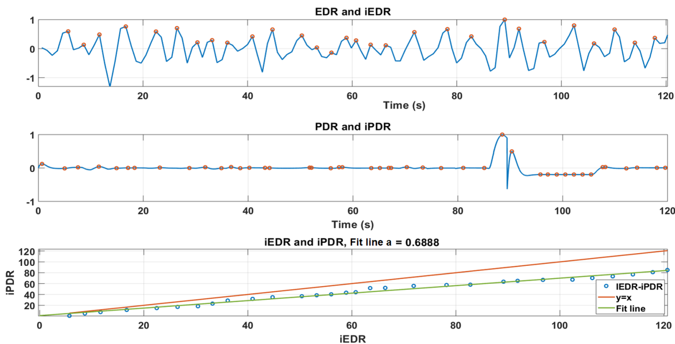
Figure 18. (Top): the EDR signal and its local maxima (peaks) iEDR . (Middle): the PDR signal and its local maxima iPDR . (Bottom): the theory fit line ( y = x ) in red and the linear regression fit line between iEDR and iPDR ( a = 0.68 ).
