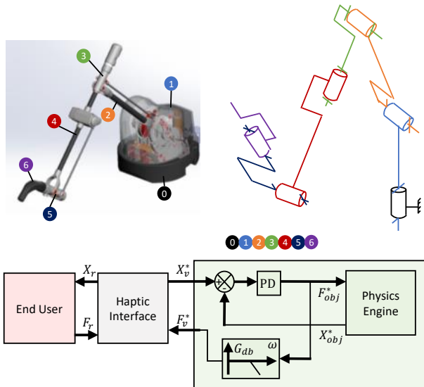
Fig. 1. Top left : Virtuouse6D 3D mock-up. Top right : Kinematic scheme of the HI. Bottom : Detailed haptic interaction. End-user interacted with the haptic display by moving the end-effector X_r . The position of each joint X_v was captured, digitalized and sent to the VE. It was coupled to the object scene through a virtual spring-damper because of the admittance control of Rigidbody, the physics engine used. The resulting force F_v^* was low-pass filtered and sent to the HI and used to apply to the end-effector as the force feedback.
