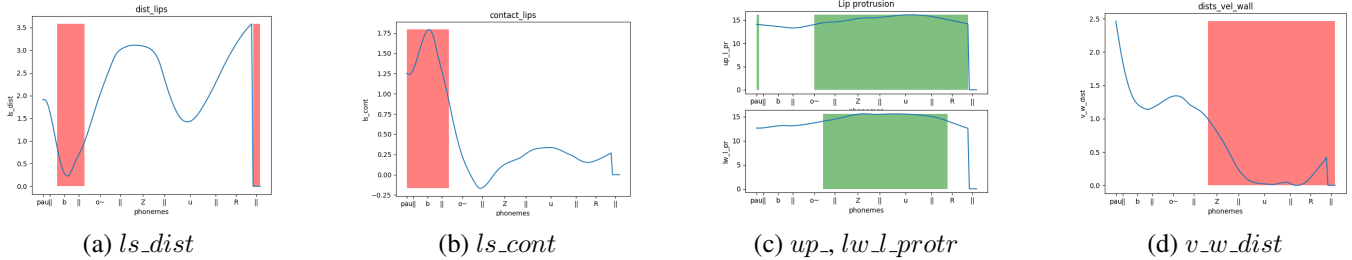
Fig. 4: Synthesis of “bonjour” /bɔ̃ʒuə/. The lip closure (4a, 4b in red) is consistent with the production of the labial stop /b/ and the narrowed labial opening for /u/ and with open lips throughout the rest of the utterance. The lips are correctly protruded (4c, green) at /ɔ̃/ and /u/. Nasality (4d, red for oral sound) is correct for all phonemes but /b/.
