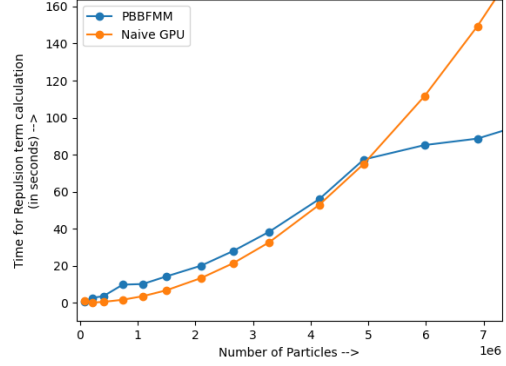
Fig. 1: Computation times for the repulsion term F^r as a function of the number of particles p .
