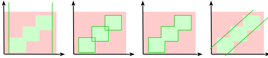
Fig. 4. Illustration of temporal discrimination power of the different instances of GDC. Planes (x, y) represent a pair of temporal constraints for some sequences (A, t_0)(B, t_0 + x)(C, t_0 + x + y) . Positive sequences are those with (x, y) values in the green region, negative sequences have (x, y) values in the red region. The bold-green lines represent the separation boundaries learned by a GDC depending on the type of occurrence assessment function, \mu . From left to right: discriminant episodes (temporal constraints with shape [0, +\infty] ), chronicles (three chronicles with temporal constraints represented by rectangles), DT-DC (a single shape combining several rectangles), linear-SVM (a single chronicle, with generalized linear boundaries).
