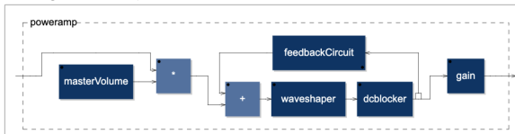
Fig. 11: Diagrams of the final implementation.
