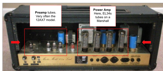
Fig. 3. The back of a Marshall JCM800 power head. We can see the two amplification stages.
