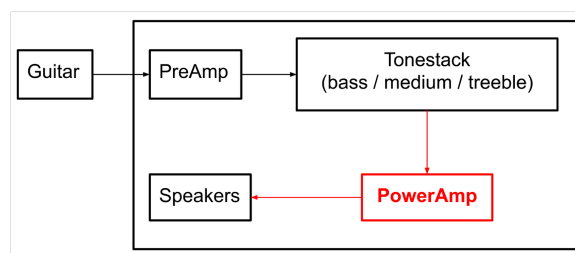
Fig. 2. The typical stages of guitar amplifiers and their associated signal paths. Some brands (as Fender) may switch the PreAmp and the Tonestack stages.
