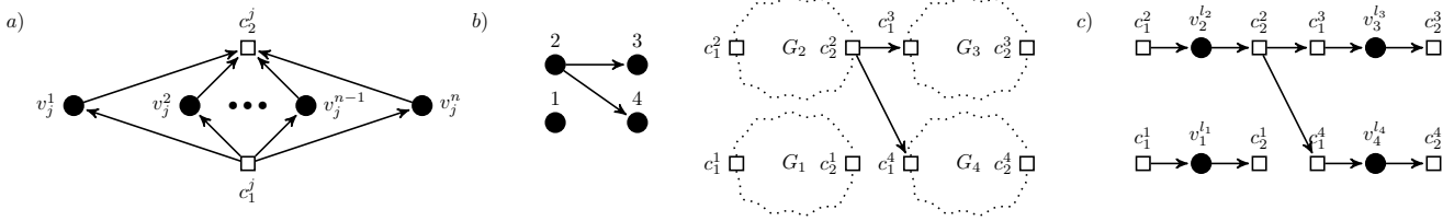
Fig. 2. Examples for the reduction of Theorem 1: a) Conditional pair as in the reduction, b) Precedence constraint graph of an LS-MAX instance and the constructed conditional DAG where each G_i is an abstraction of a conditional pair as illustrated in a), and c) Realization G'_j of the conditional DAG in b).
