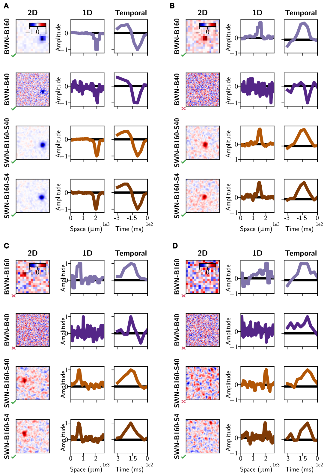
Figure 3: STAs representatives examples for four neurons, showing different situations in terms of RF mapping depending on the stimulus. The representation is the same as in Fig. 3. A green tick icon (resp. a red cross icon) is used to indicate that the RF was mapped or not. In general, SWN yields to smoother spatial STAs than the BWN, without changing the temporal STA.
