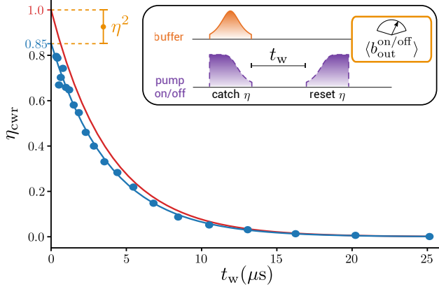
FIG. 3. Red solid line: round trip efficiency \eta_{\text{CWR}} as a function of the waiting time t_w assuming that the only imperfection comes from the memory decay with a characteristic time T_{1,m} . Blue dots: lower bound on the measured round-trip efficiency \eta_{\text{CWR}} . Blue solid line: exponential decay with characteristic time T_{1,m} . Orange error bar: range of possible values for \eta^2 that leads to a catch efficiency \eta = 0.96 \pm 0.04 . Inset: pulse sequence of the catch-wait-release protocol. We measure the average outgoing amplitude \langle b_{\text{out}}^{\text{on/off}} \rangle when the pump is on or off, from which we compute the round trip efficiency \eta_{\text{CWR}} = \langle b_{\text{out}}^{\text{on}} \rangle^2 / \langle b_{\text{out}}^{\text{off}} \rangle^2 .
