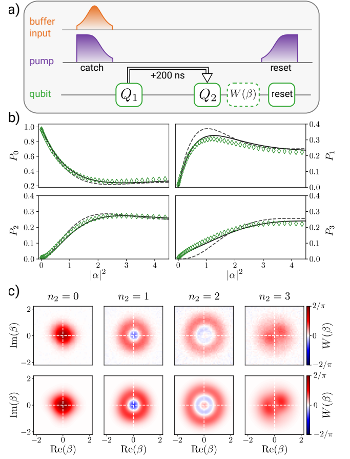
FIG. 5. Photocounting coherent states. a) Pulse sequence showing an incoming mode on the buffer with a coherent state of amplitude \alpha and the optimal shape of the pump to catch the wavepacket with minimal distortion (Appendix D). The qubit performs photocounting bit by bit with pulse sequences Q_k 's described in Fig. 4. Q_2 uses the outcome of Q_1 in a feedback protocol that adds as little as 200-ns delay. Finally, a direct Wigner tomography of the memory can be performed [45–47] before the memory and qubit are reset. b) Green diamonds: measured probabilities P_{n_2} of finding a number n_2 = n \bmod 4 photons as a function of the mean photon number |\alpha|^2 of the incoming coherent state after 200000 runs of the sequence. Dashed lines: modulo-4 Poisson distribution. Solid lines: master-equation solution without any free parameter. c) Corresponding measured (top) and simulated (bottom) Wigner functions for \alpha = \sqrt{0.5} mean photons (Appendices F and G). From left to right, the Wigner function is heralded on the counter outcome n_2 = 0, 1, 2 , and 3 out of a total of 44000 realizations per pixel.
