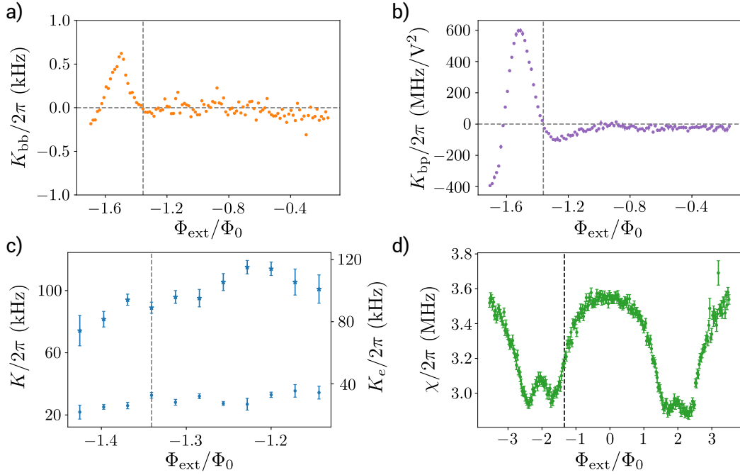
FIG. 8. Rates of nonlinear terms in the device as a function of the external flux \Phi_{\text{ext}} . Notice that the flux range is different for each panel. a) Buffer self-Kerr rate K_{bb} , b) Pump-buffer cross-Kerr rate K_{bp} , c) Dots, memory self-Kerr rate K , stars, nonlinear rate K_e . d) Dispersive shift \chi between qubit and memory.
