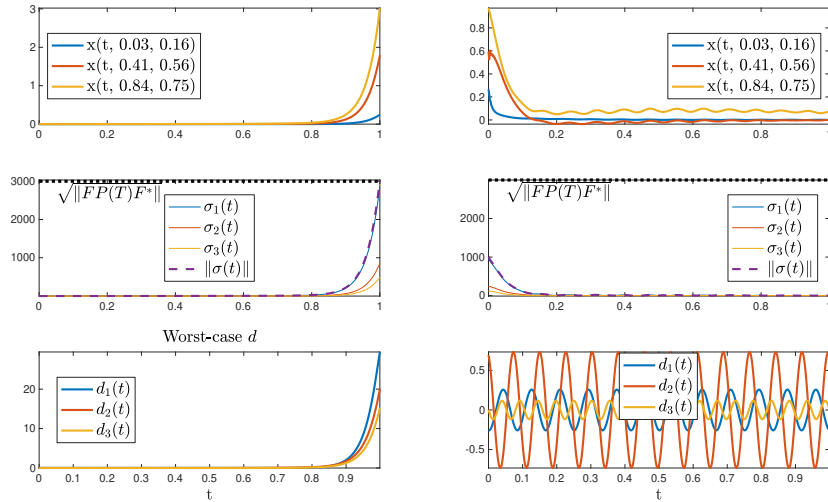
Figure 2: As in Figure 1, the left column demonstrates the worst case, whereas the right column demonstrates some arbitrary values for d, w, x_0 . The top panels show the values of x(t) in 3 locations within \Omega , whereas the middle shows the components \sigma_i(t) , i = 1, 2, 3 , of the sliding variable, as well as its norm, and we see that also in this case, the worst-case bound is reached as claimed, and the arbitrary case stays well below it. The observations were generated setting \bar{c} = 1 in every 2nd grid-point of \Omega .
