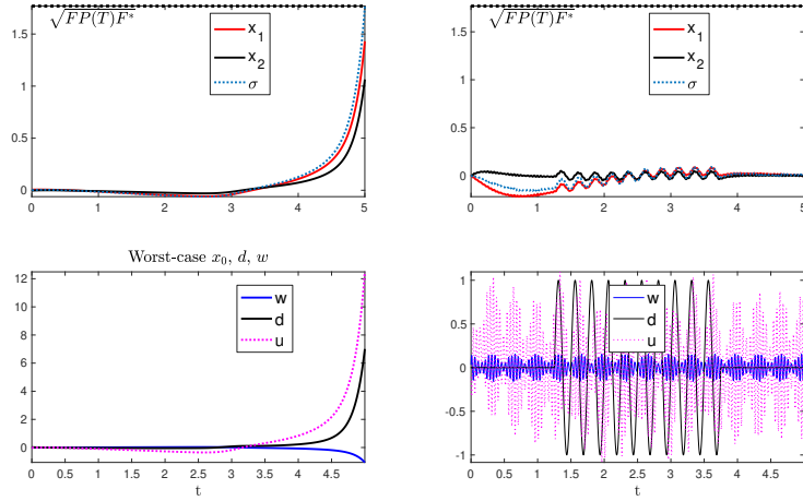
Figure 1: Closed-loop behaviour of the delayed differential equation (32) when coupled with the proposed controller. The top panels show the trajectories of x_1 and x_2 as well as the sliding variable \sigma resulting if the disturbance d and measurement noise w are as shown in the bottom panels. The control input u_{eq} is also shown in the bottom panels. The panels on the left demonstrate the worst-case d and w (and also initial state x_0 , which is not shown) in the ellipsoid (4), as given in (15); i.e. \sigma(T) should equal its largest possible value. As can be seen, \sigma(T) = \sqrt{FP(T)F^*} , as claimed in (29) in Corollary 2. The panels to the right demonstrate the case of an arbitrary, non-worst-case realization of w, d and x_0 ; we see that the control u_{eq} is effective in steering \sigma close to zero, and that the actual \sigma is way below the worst-case bound (29).
