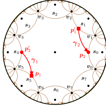
(b) Sequence of oriented hyperbolic line segments.
