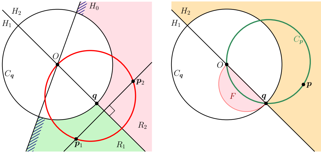
Figure 22: Illustrations for the proof of Lemma 25.
