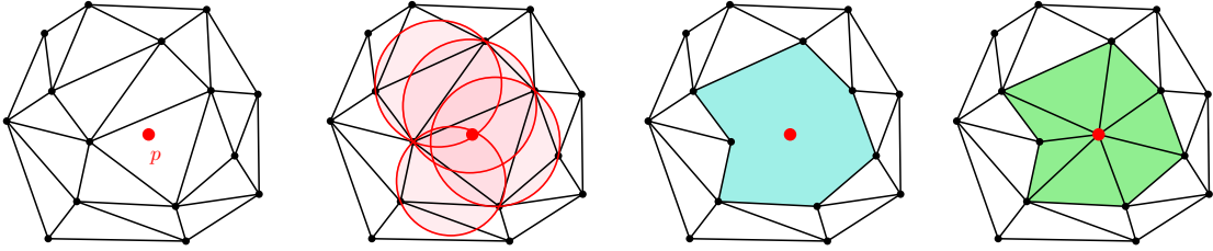
Figure 4: Insertion of a point in a Delaunay triangulation with Bowyer's incremental algorithm.
