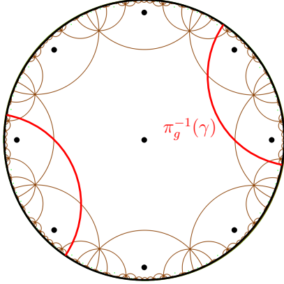
(a) Preimage of a closed geodesic \gamma on the Bolza surface.
