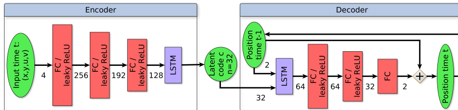
Figure 1: Recurrent auto-encoder network computing the latent representation of trajectories. Numbers indicate the input dimension for each layer.
