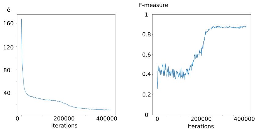
Figure 11: Evolution of the trajectory reconstruction error \bar{\epsilon} (left) and of the F-measure related to trajectory saliency detection (right) on the validation set of the STMS dataset during training. Each iteration corresponds to a batch of 60 to 66 trajectories (depending on the random inclusion of salient trajectories).
