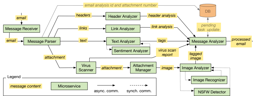
Fig. 4 Microservice architecture for email processing pipeline.
