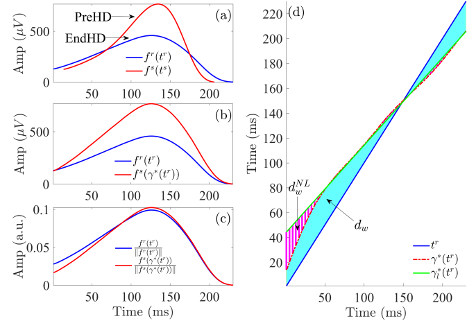
Fig. 2. Linear and non-linear time warping for a patient. Panel (a) shows reference (blue) and investigated (red) T waves obtained from an ECG segment during HD. Panel (b) shows the warped T waves, which have the same duration while keeping the original amplitude. Panel (c) depicts the warped T waves after normalization by their L2-norms. The area (cyan region) between both T waves in panel (d) represents d_w , which quantifies the total amount of warping. The light green solid line is the linear regression function \gamma_l^*(\mathbf{t}^r) best fitted to \gamma^*(\mathbf{t}^r) . The marker d_w^{\text{NL}} quantifies the non-linear warping by computing the area of the dashed purple region between \gamma^*(\mathbf{t}^r) and \gamma_l^*(\mathbf{t}^r) .
