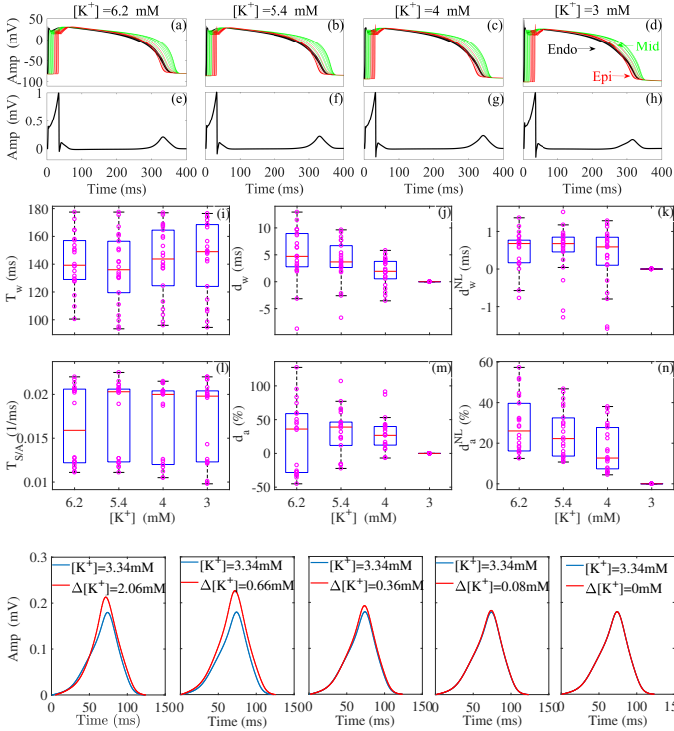
Fig. 4. Panels a-d: Simulated endocardial (black), midmyocardial (green) and epicardial (red) APs for simulated fiber C154, and \mathcal{F}\{[K^+]; 2.0 \text{ mM}; 1.0 \text{ s}\} . Panels e-h: ECGs for varying [K^+] . Panels i-n: Changes in T_w , T_{S/A} , d_w , d_a , d_w^{NL} and d_a^{NL} for simulated fibers when varying [K^+] . Central red lines indicate the median, whereas bottom and top edges show the 25th and 75th percentiles, respectively. Each purple dot corresponds to an individual simulated fiber. In the bottom panels, red traces indicate the T waves of a simulated fiber from an initial (maximum) to a final (minimum) value of [K^+] corresponding to average [K^+] values in the analyzed patients. The blue line indicates the reference T wave used when computing time-warping markers.
