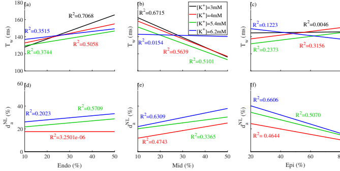
Fig. 7. Panels a-c: Fitted regression lines for the average values of T_w for all simulated cases sharing the same proportion of endocardial, midmyocardial or epicardial cells at different [K^+] levels. Panels d-f: Fitted regression lines for the average values of d_a^{NL} for all simulated cases sharing the same proportion of endocardial, midmyocardial or epicardial cells at different [K^+] , with the reference value for [K^+] = 3 mM. Coefficients of determination ( R^2 ), estimated as the square of the linear correlation coefficient between the analyzed T wave markers and each cell type (endocardial, midmyocardial or epicardial), are indicated.
