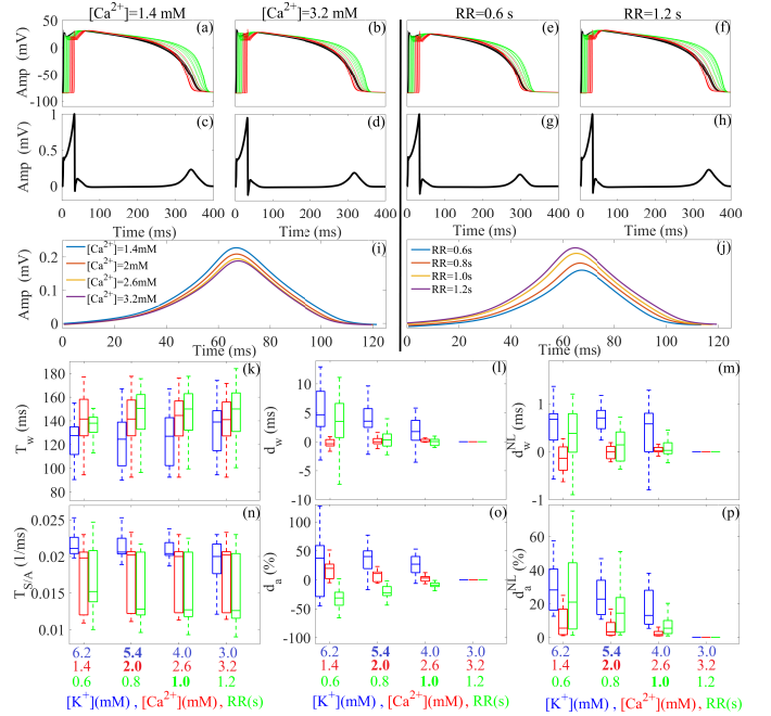
Fig. 5. Panels a, b: Simulated endocardial (black), midmyocardial (green) and epicardial (red) APs for simulated fiber C154, \mathcal{F}\{5.4 \text{ mM}; [Ca^{2+}]; 1.0 \text{ s}\} under varying [Ca^{2+}] . Panels c, d: ECGs and T waves for [Ca^{2+}] variations. Panels e, f: Simulated endocardial (black), midmyocardial (green) and epicardial (red) APs for simulated fiber C154, \mathcal{F}\{5.4 \text{ mM}; 2.0 \text{ mM}; RR\} , under varying RR. Panels g, h, j: ECGs and T waves for RR variations. Panels i, k-p: Changes in T_w , T_{S/A} , d_w , d_a , d_w^{NL} and d_a^{NL} for varying [K^+] , \mathcal{F}\{[K^+]; 2.0 \text{ mM}; 1.0 \text{ s}\} (blue boxplots), [Ca^{2+}] , \mathcal{F}\{5.4 \text{ mM}; [Ca^{2+}]; 1.0 \text{ s}\} (red boxplots), and RR, \mathcal{F}\{5.4 \text{ mM}; 2.0 \text{ mM}; RR\} (green boxplots), in the horizontal axis for the 22 simulated fibers. Central lines indicate the median, whereas bottom and top edges show the 25th and 75th percentiles, respectively. Values of [K^+] \in \{3.0, 4.0, 5.4, 6.2\} \text{ mM} , [Ca^{2+}] \in \{1.4, 2.0, 2.6, 3.2\} \text{ mM} , and RR \in \{0.6, 0.8, 1.0, 1.2\} \text{ s} are used.
