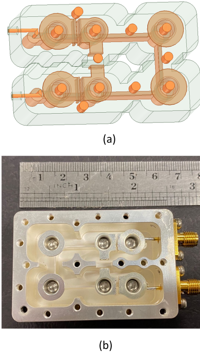
Fig. 12. (a) EM designed model of the filter with 2 dispersive couplings and a symmetric quadruplet. (b) Photograph of the prototyped filter.
