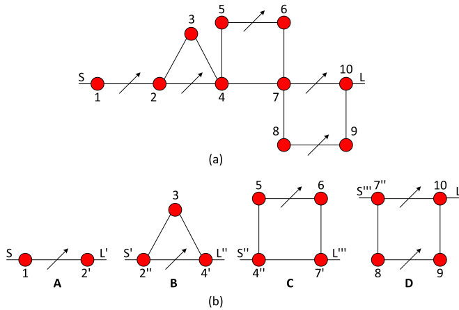
Fig. 14. (a) Topology of a ten-pole filter with the 4 dispersive blocks. (b) Separating the filter in (a) into 4 sub-filters labeled A, B, C, and D.
