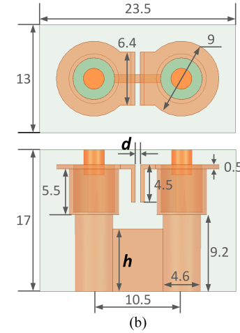
Fig. 10. (a) EM model of the dispersive coupling structure between two coaxial resonators. (b) Top and front views of the dispersive coupling structure shown in (a).
