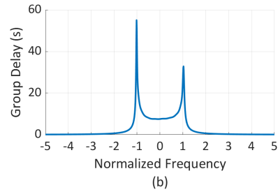
Fig. 15. (a) Response and (b) group delay of the synthesized dispersive coupling matrix ( \mathbf{Md} , \mathbf{Mo} , \mathbf{B} ).
