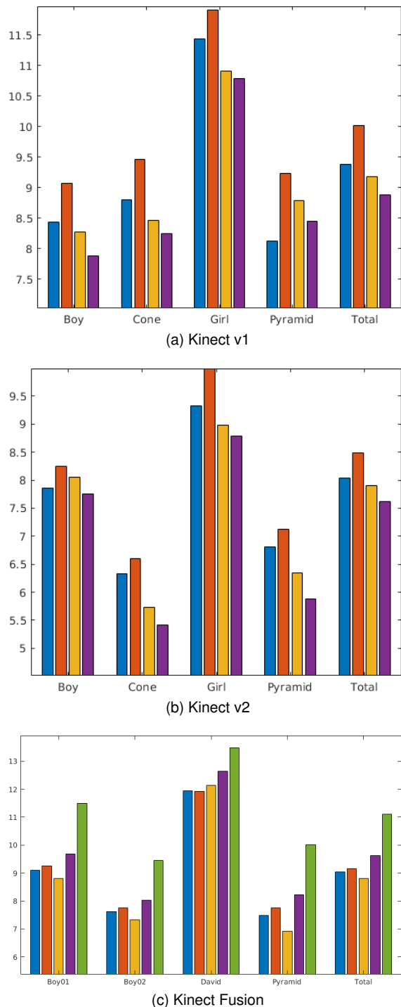
Fig. 10. Average angular errors in degrees, on the 3 Kinect datasets of [2], per scanned model. (blue) CNR. (orange) NormalF-Net. (yellow) Ours (raw estimated normals). (purple) Ours (refined normals). (green) NLLR.
