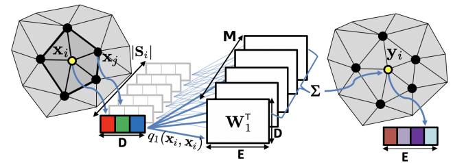
Fig. 3. The graph convolutional layer from [5], which we adapt to faces instead of vertices.
