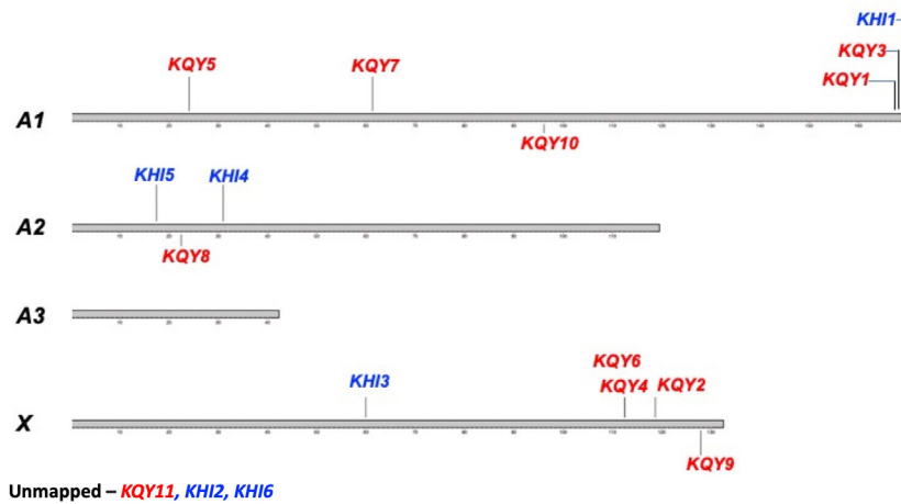
FIGURE 3 | Placement of the KQY and KHI genes on the pea aphid chromosomes. The pea aphid chromosomes A1, A2, A3, and X. KQY genes are colored in red and the KHI genes are colored in blue. KQY11, KHI2, and KHI6 are unmapped.
