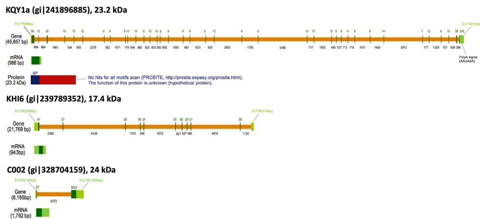
FIGURE 4 | Gene structures of KQY1a and KHI6. C002 is shown for comparison. Diagrams are based on the graphic sequence display generated from the NCBI genome sequence viewer. Orange bars = introns; Green bars = exons.
