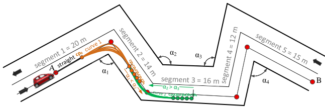
(a) Algorithm searches the best location for the junction point between curves in real-time
