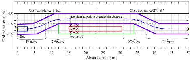
FIGURE 7: Virtual lane generation for moving obstacles considering the obstacle's occupied space prediction
