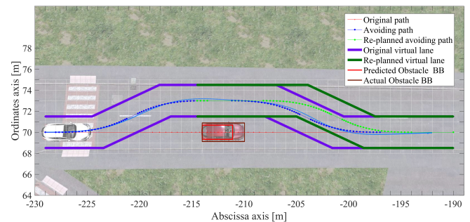
FIGURE 9: Planned path and metrics for evaluating the proposed approach in a static environment
