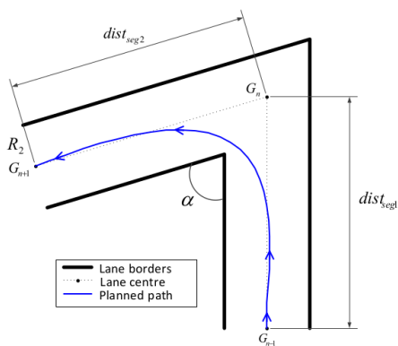
FIGURE 2: Single-turn scenario with optimal curve search [34]
