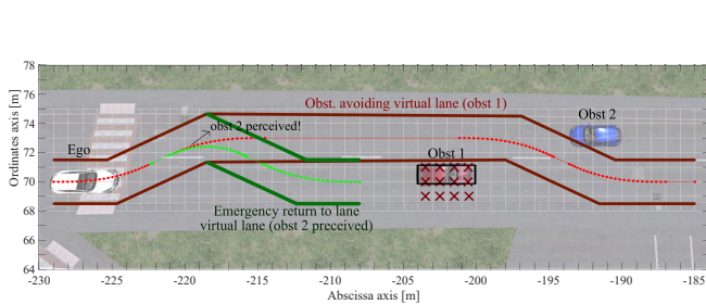
(a) Obstacle avoiding and re-computed emergency return to the lane paths and virtual lanes
