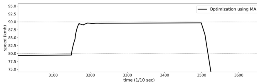
Figure 5. Detail of the performance of MA in one step response.
