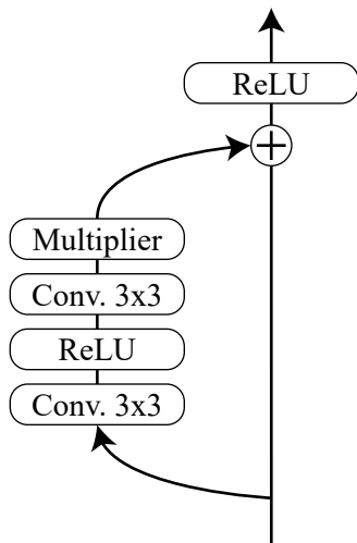
Fig. 2. Scheme of a single residual block.
