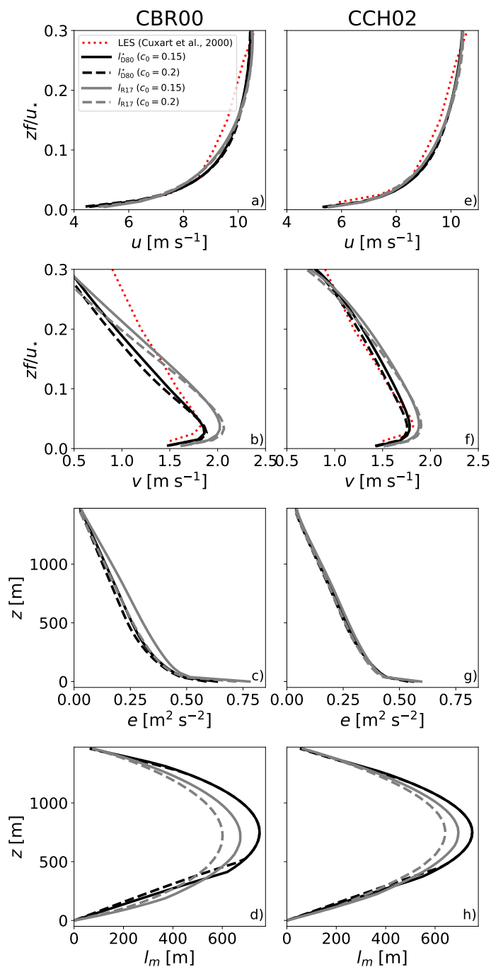
Figure 4. Results obtained for the neutral boundary-layer case of Andren et al. (1994) with the CBR00 model constants (left panels a to d) and CCH02 model constants (right panels e to h) for different parameter values for c_0 and different mixing length formulations ( l_{D80}^+ for black lines or l_{R17} for grey lines). Results are shown for u (panels a & e), v (panels b & f), e (panels c & g), and l_m (panels d & h). In the top four panels results are compared with LES simulations from Cuxart et al. (2000) (their Fig. 16). As in Andren et al. (1994), simulations were run over a period of 10/f and results are averaged over the last 3/f period.
