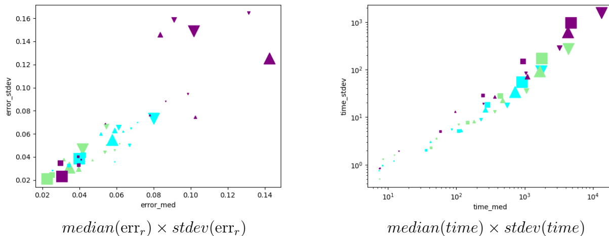
Figure S 1: Estimating the volume of three polytopes with known volumes (cube, isotropic simplex, standard simplex), in dimension n = 10, 30, 50, 70, 100 , with three algorithms. Statistics reported over 50 runs. The error of an estimate \tilde{V} is defined as err_r = |\tilde{V} - V|/V . Symbol shape vs polytope: square: cube; triangle up: isotropic simplex; triangle down: standard simplex Symbol size vs dimension : smallest for n = 10 , largest for n = 100 Color vs algorithm: purple/light blue/light green HAR/HMC0/HMC1.5
