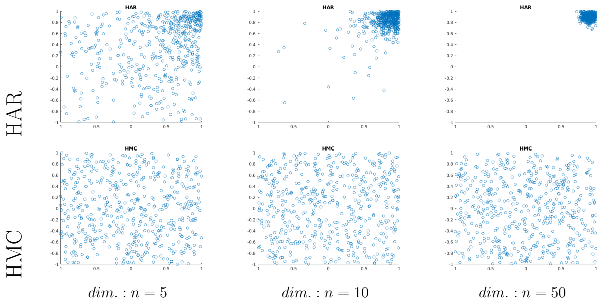
Figure 3: HMC for the cube [-1, 1]^n : ability to escape corners, and comparison to Hit-and-run. A nearly flat isotropic Gaussian was used to approach the uniform distribution ( \sigma = \sqrt{500} ). For n > 3 , the plot displays projections onto the first two coordinates. Simulations were started from a corner ( q_i^{(0)} = 0.9 ). Samples generated after 10 steps of HAR or HMC, repeated 500 times – whence 500 samples.
