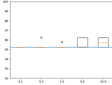
Fig. 20: Accuracy of the classifier after retraining with 25 adversarial configurations in the training set over a test set of about 89,000 configurations. The blue line reports the baseline accuracy of the classifier when no adversarial configurations are added to the training set.
