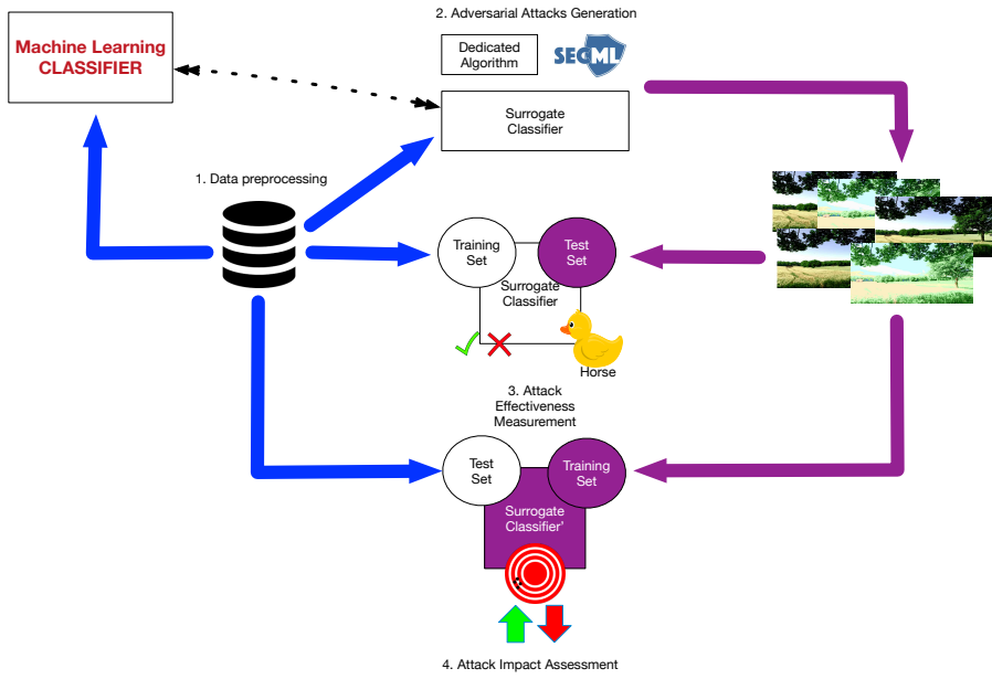
Fig. 4: Adversarial Pipeline
