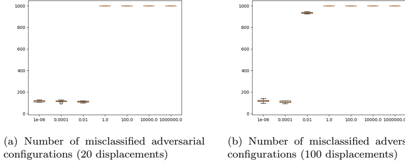
Fig. 17: Number of successful attacks on class not building ; X-axis represents different step size values t while Y-axis is the number of misclassified adversarial configurations by the classifier.
