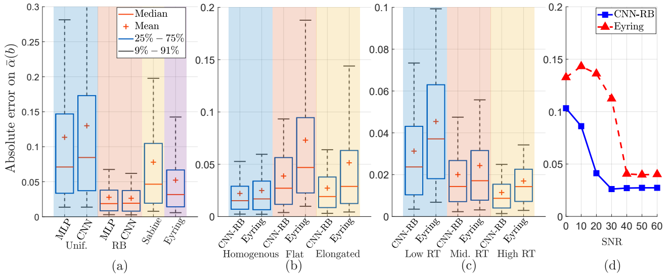
Figure 1. Errors on mean absorption coefficients using the proposed neural networks (MLP, CNN) trained on two datasets (Unif., RB) vs. reverberation theory (Sabine, Eyring). (a) Realistic absorption profiles, (b) Homogenous vs. flat vs. elongated room geometries, (c) RT_{60}(b) < 0.5 s vs. RT_{60}(b) \in [0.5, 1.5] s vs. RT_{60}(b) > 1.5 s, (d) Varying SNR.
