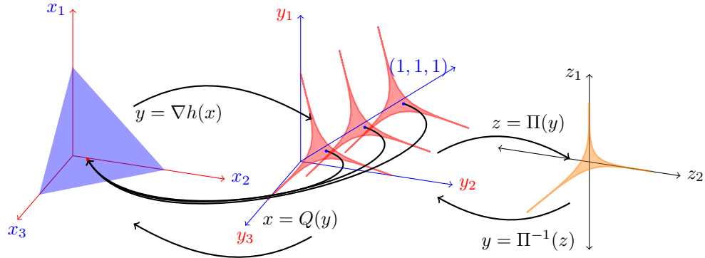
Figure 5: The three different representation spaces of (FTRL): primal (strategies, left); dual (payoffs/scores, center); dual quotient (payoff/score differences, right).
