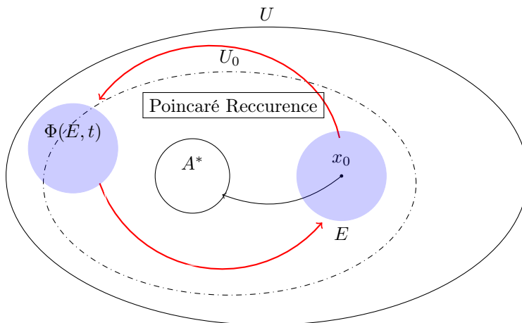
Figure 6: The various sets in the proof of Theorem C.1 .
