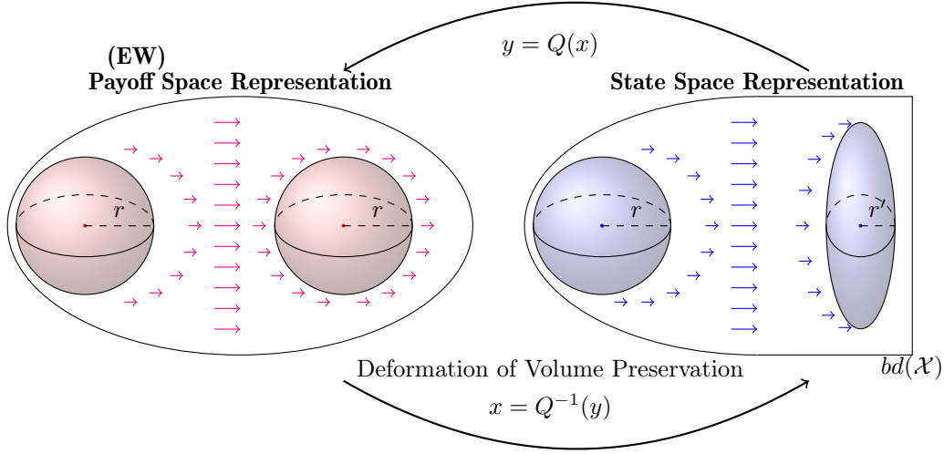
Figure 4: From payoffs to strategies and back, the steep case: deformation of neighborhoods under the logit map Q = \Lambda .
