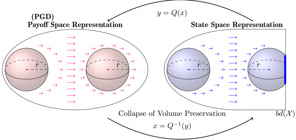
Figure 7: From payoffs to strategies and back, the non-steep case: deformation of neighborhoods under the Euclidean projection map Q = \Pi .
