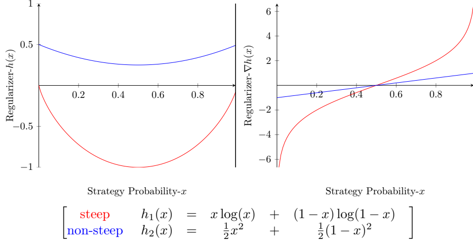
Figure 3: Steep vs. non-steep regularizers (note in particular the singular behavior of the gradient at the boundary in the case of steep regularizers).
