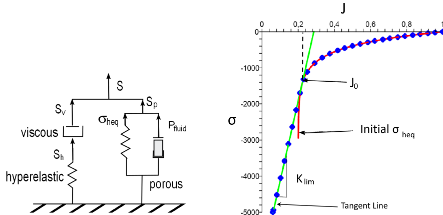
Figure 3: (Left) Representation of the constitutive model combining viscosity, hyperelasticity and porosity. (Right) Representation of the static Cauchy stress before and after substitution leading to the final dotted curve. Here f_w = 0.8 .
